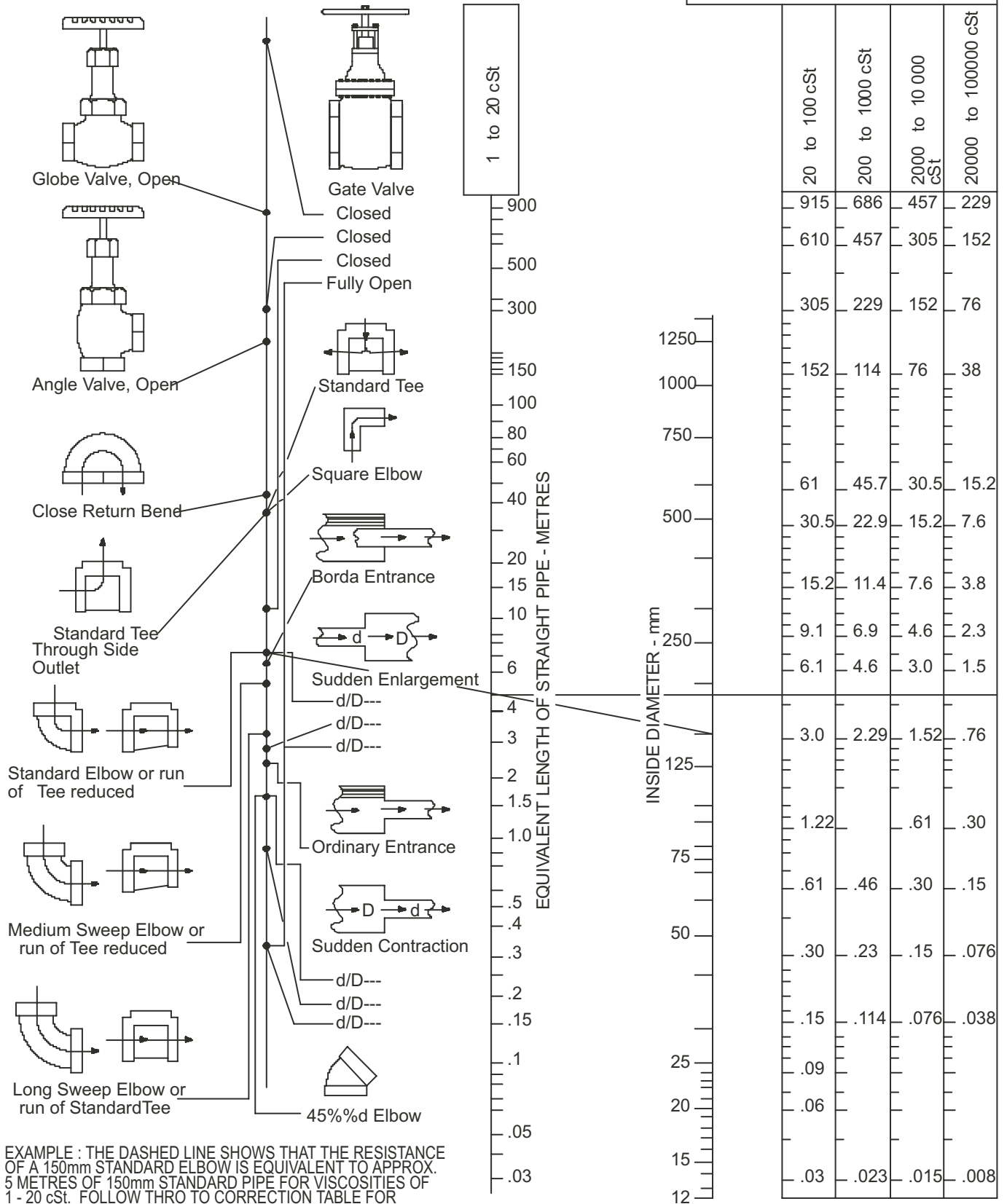
EQUIVALENT LENGTH OF PIPE FOR VISCOSITY RANGE (METRES)
